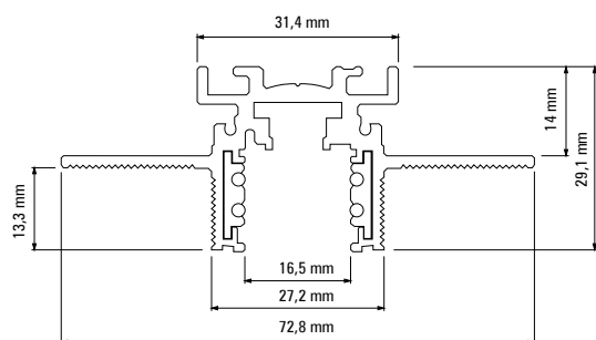
LTS 511 Low aluminum profile for recessed mounting
